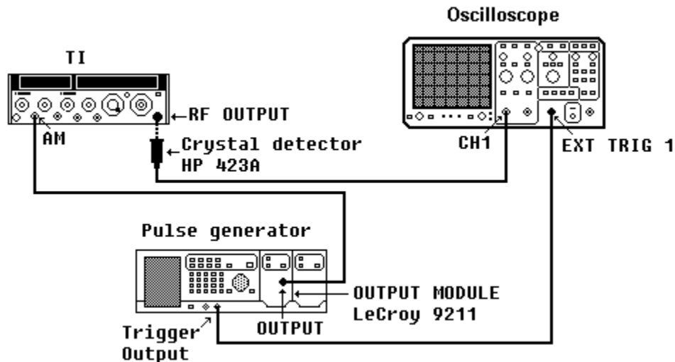
Figure 4. Doubler gain - adjustment setup
